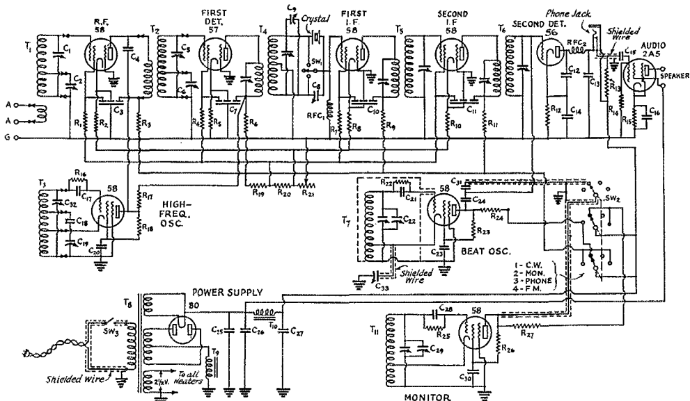
FIG. 1—THE CIRCUIT OF THE COMPLETE RECEIVER
